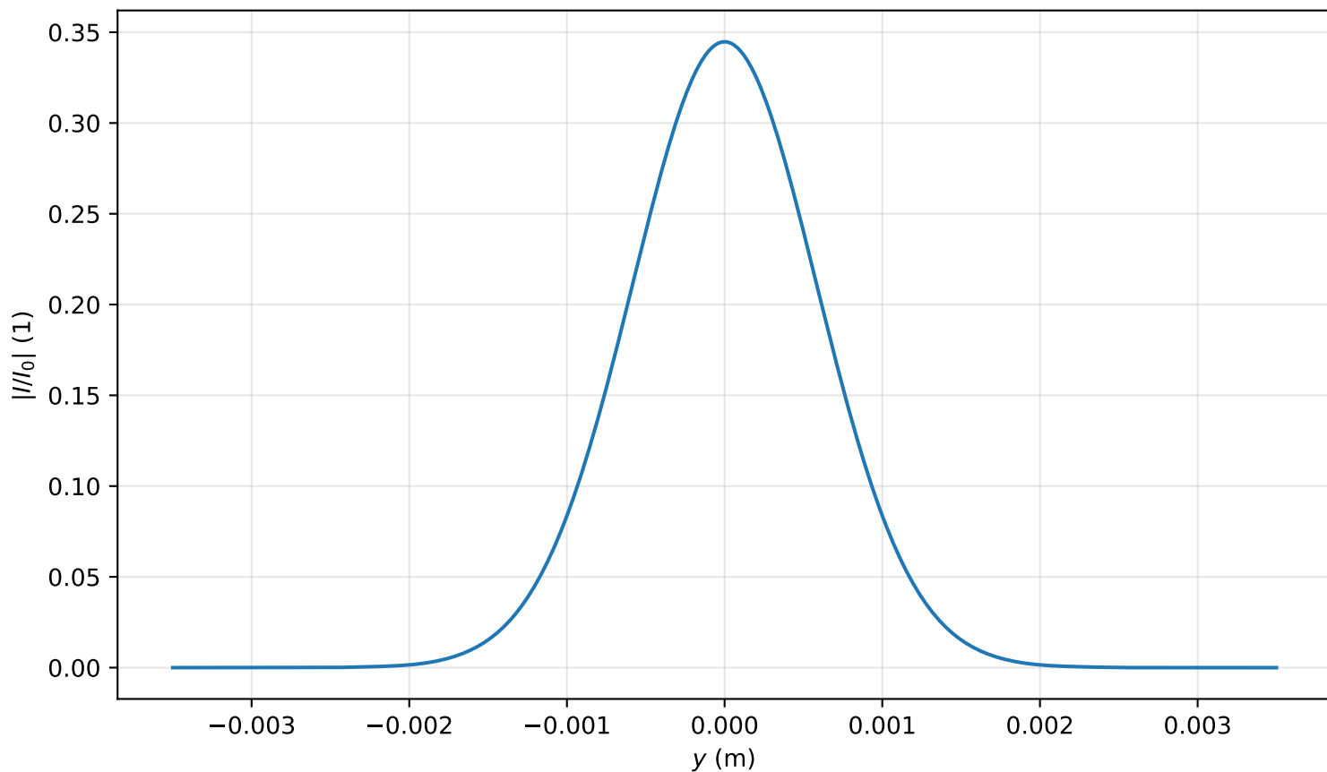
Intensity profile I(x=0, y, z=2.946)/I_0 , P_{in}=0.1P_{cr} , artificial time
